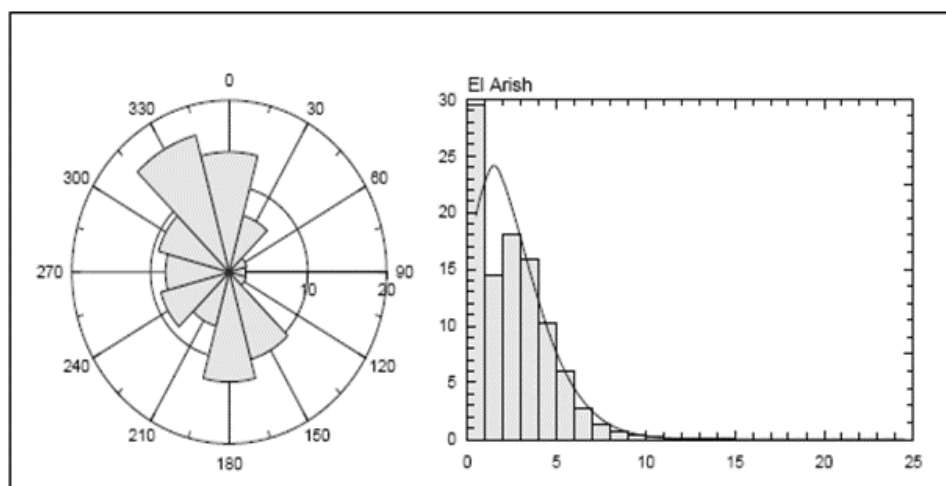
Figure 4. a- The wind
