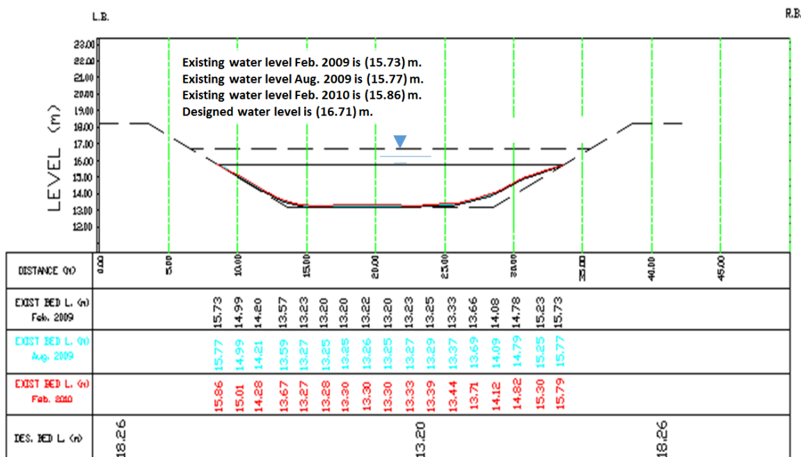
Figure 9. Actual and design cross sections for El-Sheikh Gaber Canal at km 73.000.
