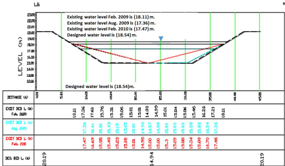
Figure 7. Actual and design cross sections for El-Sheikh Gaber Canal at km 53.000
