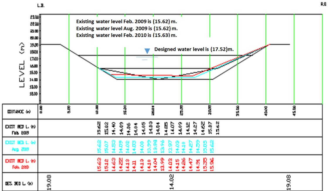
Figure 8. Actual and design cross sections for El-Sheikh Gaber Canal at km 83.000.
