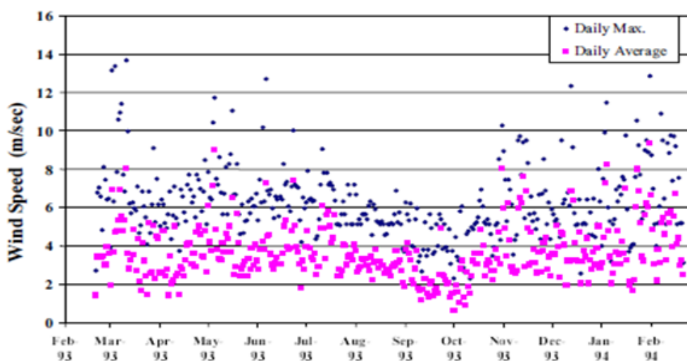
Figure 5. Average of the daily mean wind speed
