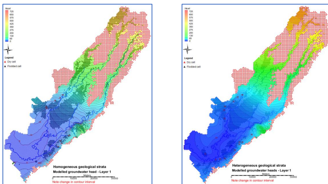
Figure 3. Head distribution in layer 1 assuming homogeneity (left) and heterogeneity (right).
