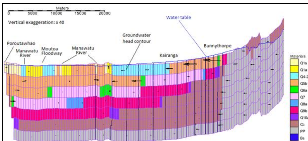
Figure 1. Transpose of lithostratigraphical units onto the groundwater model finite difference grid.
