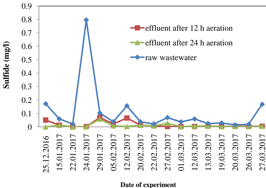
Figure1. Sulfides in wastewater and effluents after 12 and 24 h of aeration at DO 2 mg/l.
