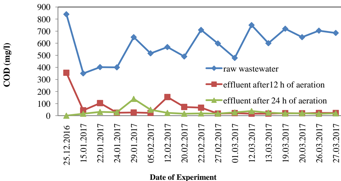
Figure 4. COD in wastewater and effluents after 12 and 24 h of aeration at DO 4 mg/l.
