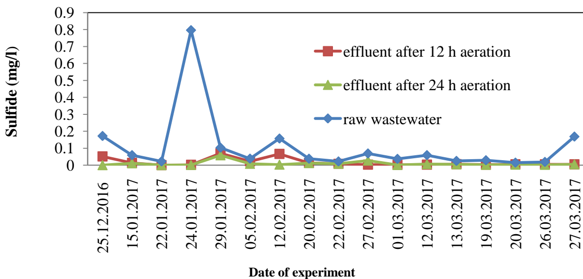
Figure1. Sulfides in wastewater and effluents after 12 and 24 h of aeration at DO 2 mg/l.
