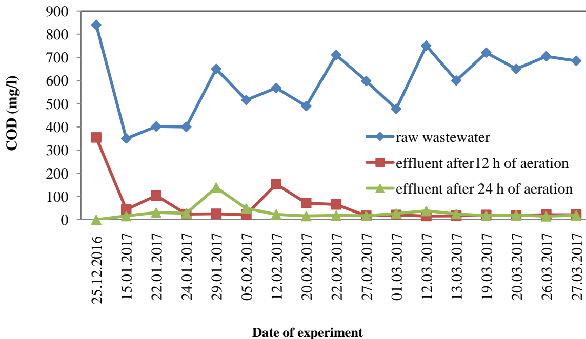
Figure 3. COD in wastewater and effluents after 12 and 24 h of aeration at DO 2 mg/l.
