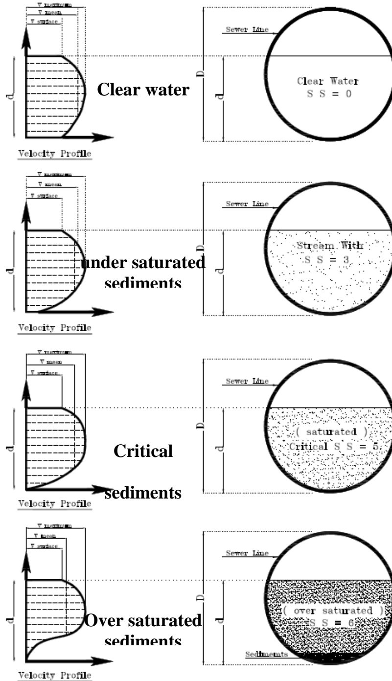
Figure 3. Velocity distribution of water with suspended sediments
