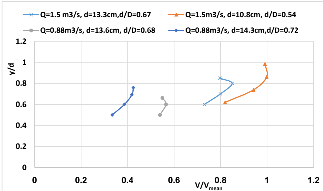
Figure (3) Dimensionless relationship between relative water depth ( y/d ) and relative velocity ( V/V_{mean} )
