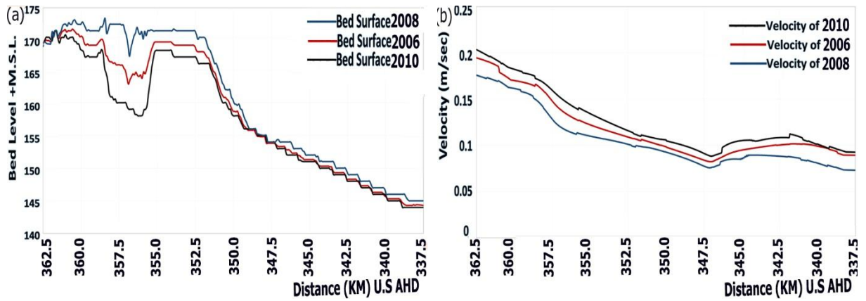
Figure 8. Comparison between bed surfaces and 2-D velocity profiles for the longitudinal section : (a) bed surfaces (b) velocity distribution, for the year 2006, 2008 and 2010.
