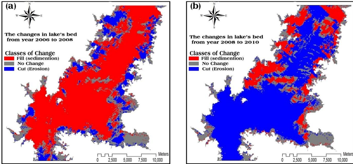
Figure 4. Typical sample for maps of changes for the years 2006-2008 and 2008-2010.
