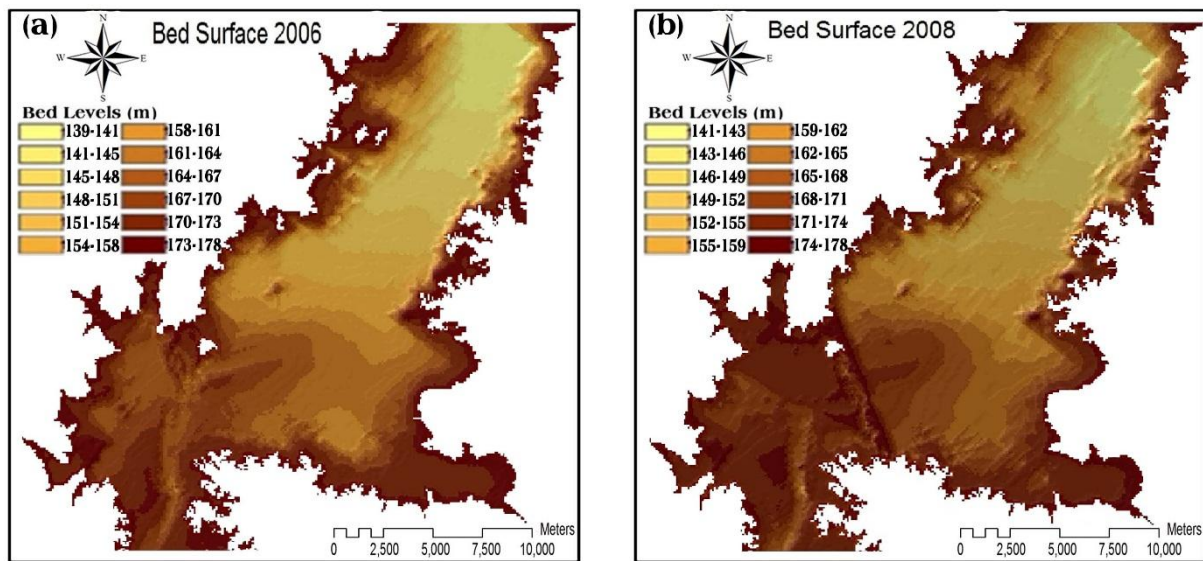
Figure 3. Typical sample results of the predicted bed surfaces for the years 2006 and 2008.
