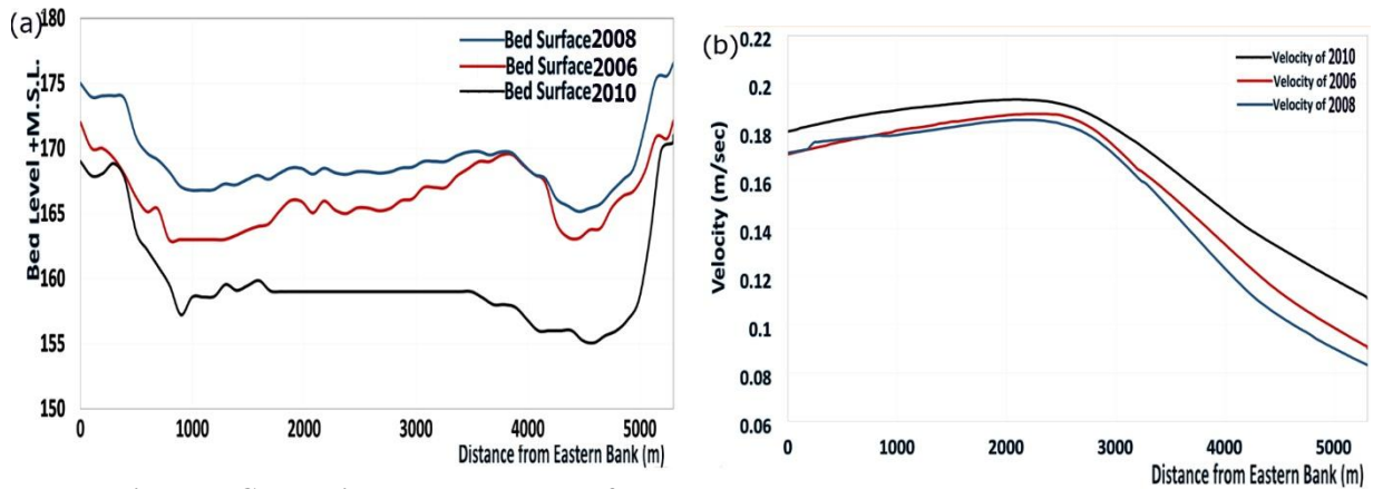
Figure 7. Comparison between bed surfaces and 2-D velocity profiles at section 26 (357 Km U.S AHD): (a) Bed surfaces cross sections; (b) Velocity distribution
