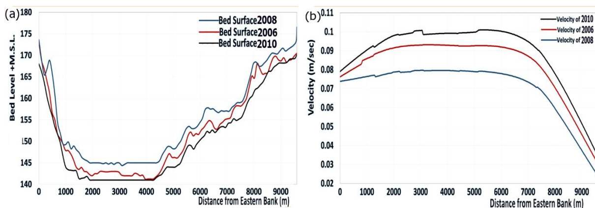
Figure 6. Comparison between bed surfaces and velocity profiles at section 22 (337.5 Km U.S AHD): (a) Bed surfaces cross sections; (b) Velocity distribution
