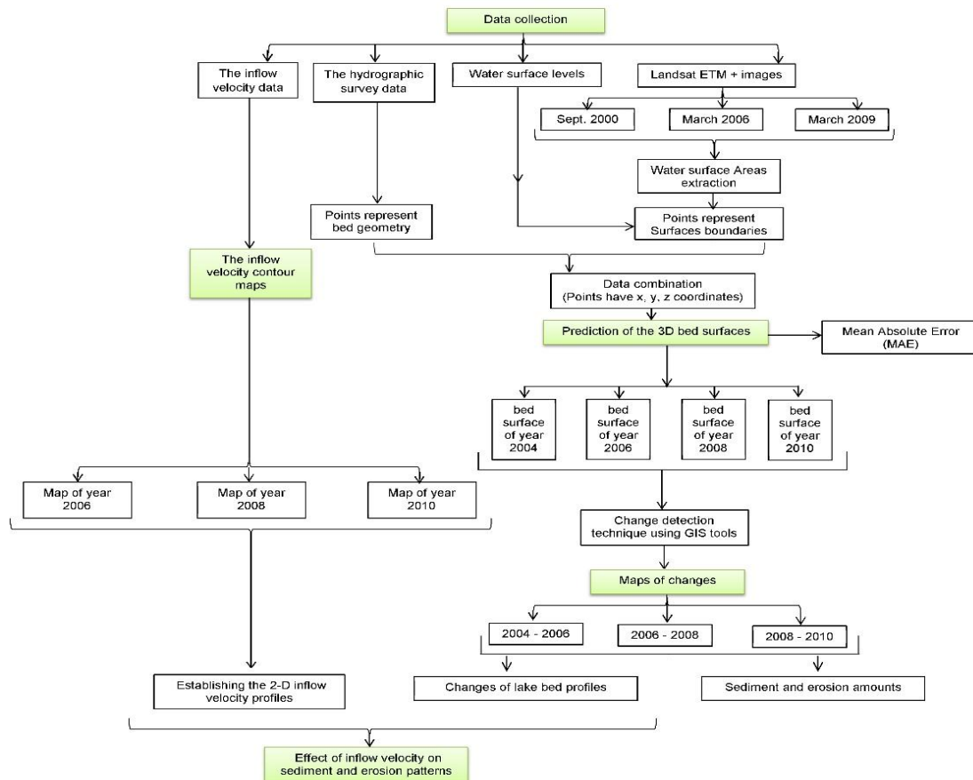
Figure 2. Flowchart of the procedures adopted to detect the correlation between the 2-D velocity profiles and sediment accumulation in the study area
