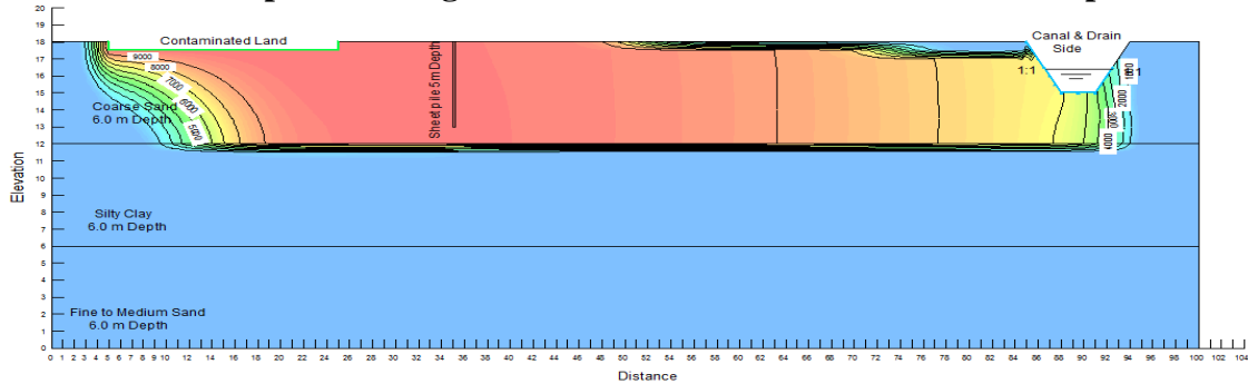
Figure 16. Contamination concentration with sheet pile, ds/Dt=0.278, X(s.p)/X(total)=0.20 and t=100 days
