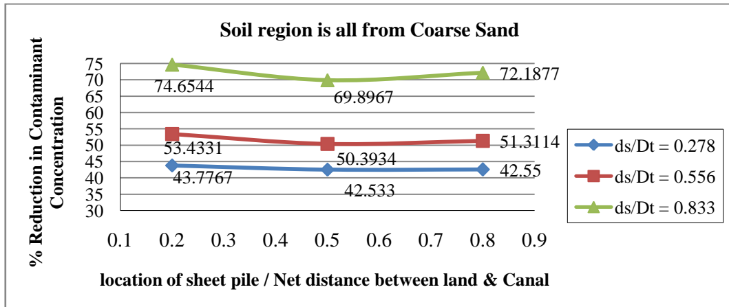
Figure 9. The reduction percentage in contamination concentration reach the toe of the slope
