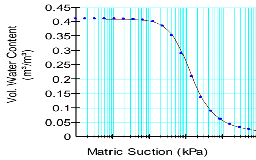
Figure 3. Vol. water content for fine to medium sand.
