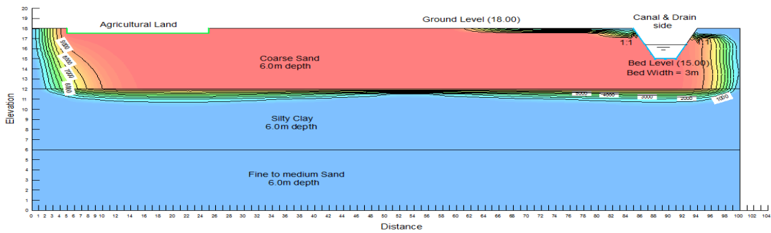
Figure 15. Contamination concentration without any sheet pile and t=100 days
