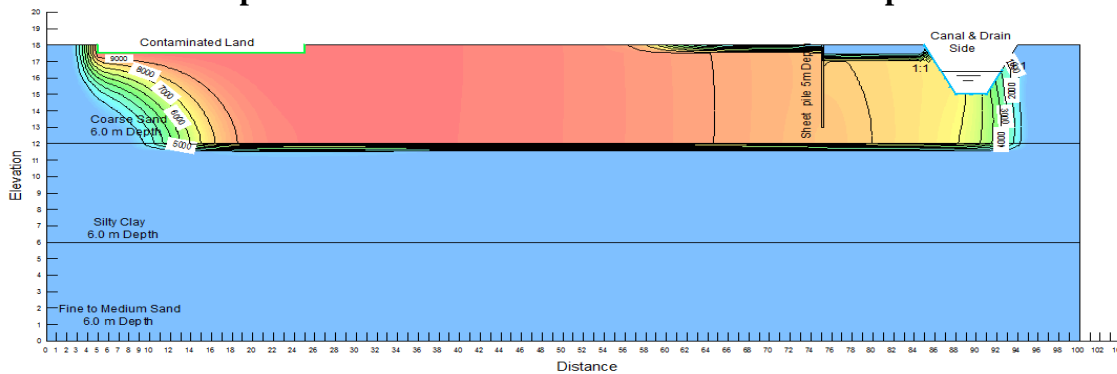
Figure 18. Contamination concentration with sheet pile, ds/Dt=0.278 , X(s.p)/X(\text{total})=0.80 and t=100 days
