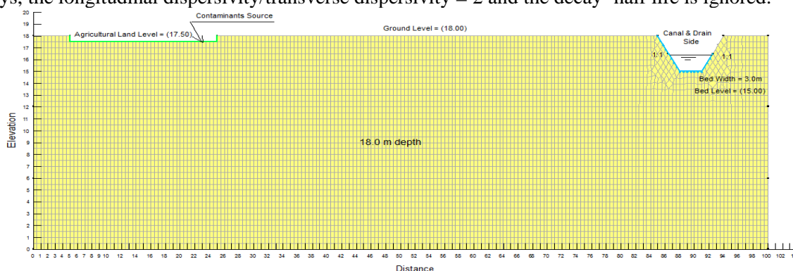
Figure 1. Model dimension and boundary conditions
