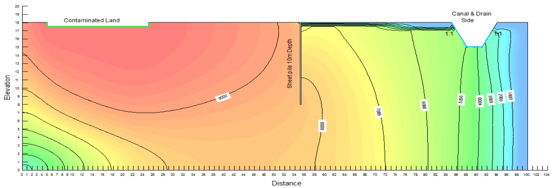
Figure 7. Contamination concentration with sheet pile, ds/Dt=0.556 , X(s.p)/X(total)=0.50 and t=100 days
