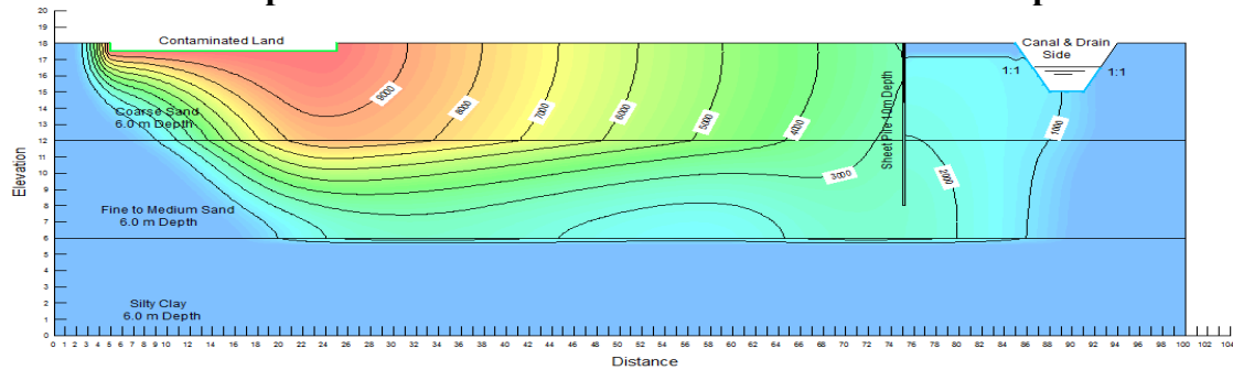
Figure 13. Contamination concentration with sheet pile, ds/Dt=0.556 , X(s.p)/X(total)=0.80 and t=200 days
