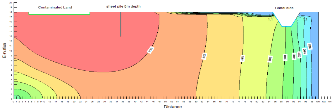
Figure 6. Contamination concentration with sheet pile, ds/Dt=0.278 , X(s.p)/X(total)=0.20 and t=100 days
