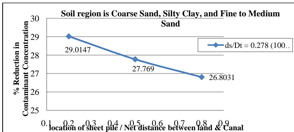
Figure 19. The reduction percentage in contamination concentration reach the toe of the slope
