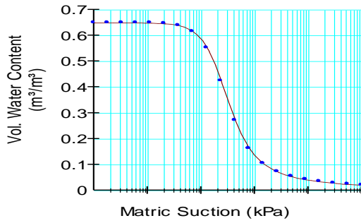
Figure 2. Vol. water content for coarse sand.
