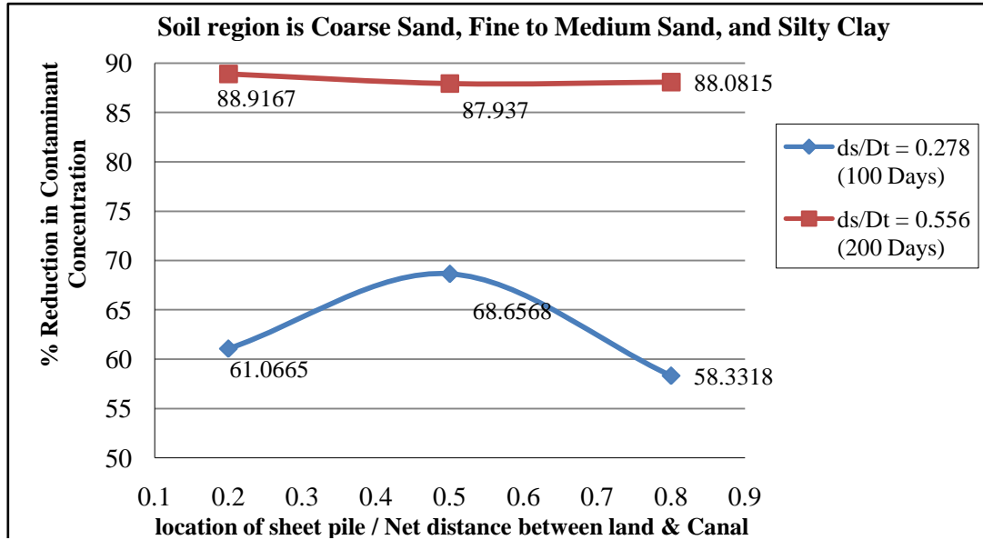
Figure 14. The reduction percentage in contamination concentration reach the toe of the slope
