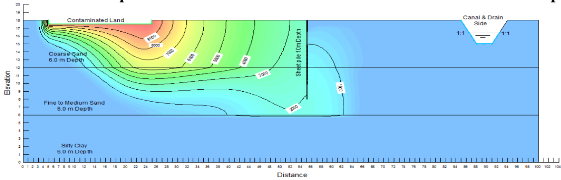
Figure 12. Contamination concentration with sheet pile, ds/Dt=0.556 , X(s.p)/X(total)=0.50 and t=100 days
