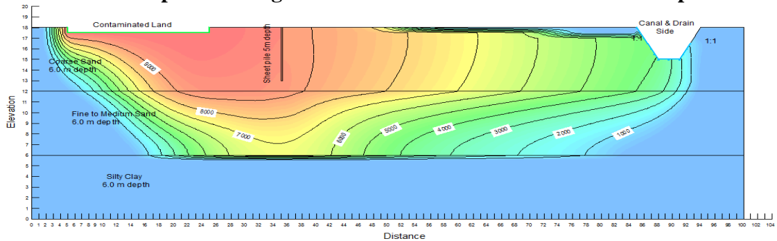
Figure 11. Contamination concentration with sheet pile, ds/Dt=0.278 , X(s.p)/X_{total}=0.20 and t=100 days
