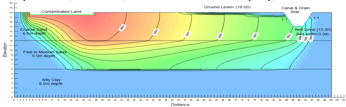
Figure 10. Contamination concentration without any sheet pile and t=100 days
