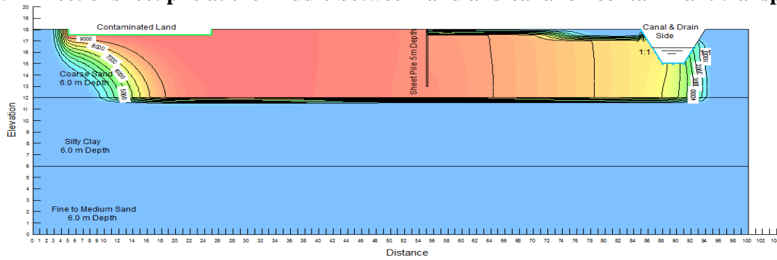
Figure 17. Contamination concentration with sheet pile, ds/Dt=0.278 , X(s.p)/X(\text{total})=0.50 and t=100 days
