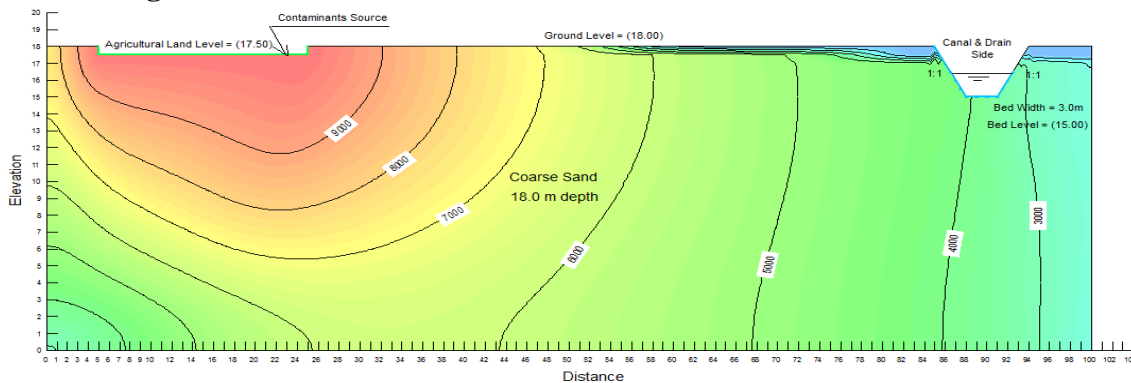
Figure 5. Contamination concentration without any sheet pile and t=100 days
