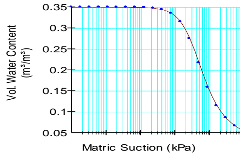
Figure 4. Vol. water content for silty clay soil.
