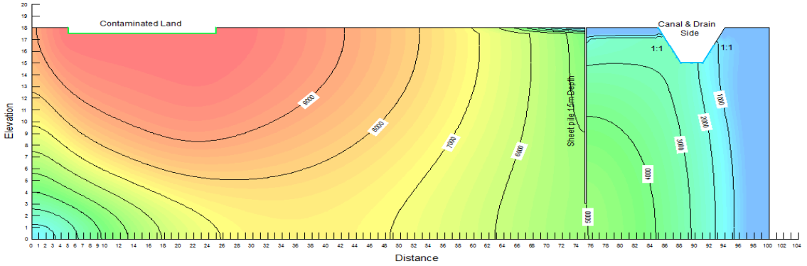
Figure 8. Contamination concentration with sheet pile, ds/Dt=0.833 , X(s.p)/X(total)=0.80 and t=100 days
