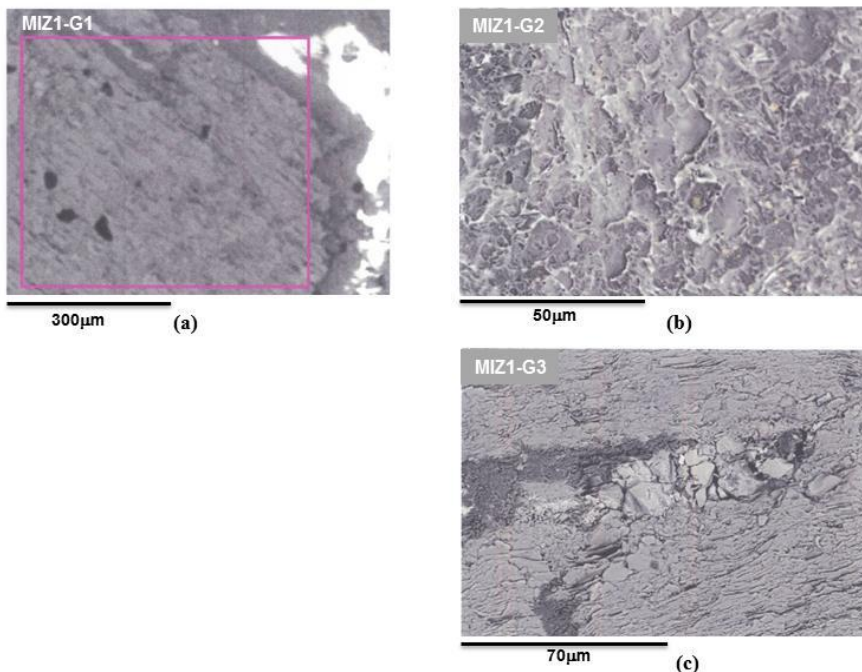
Figure 6. SEM images of granitic samples before and after water-rock interaction test a) Unaltered reacted sample b) Altered reacted sample c) Altered not reacted sample
