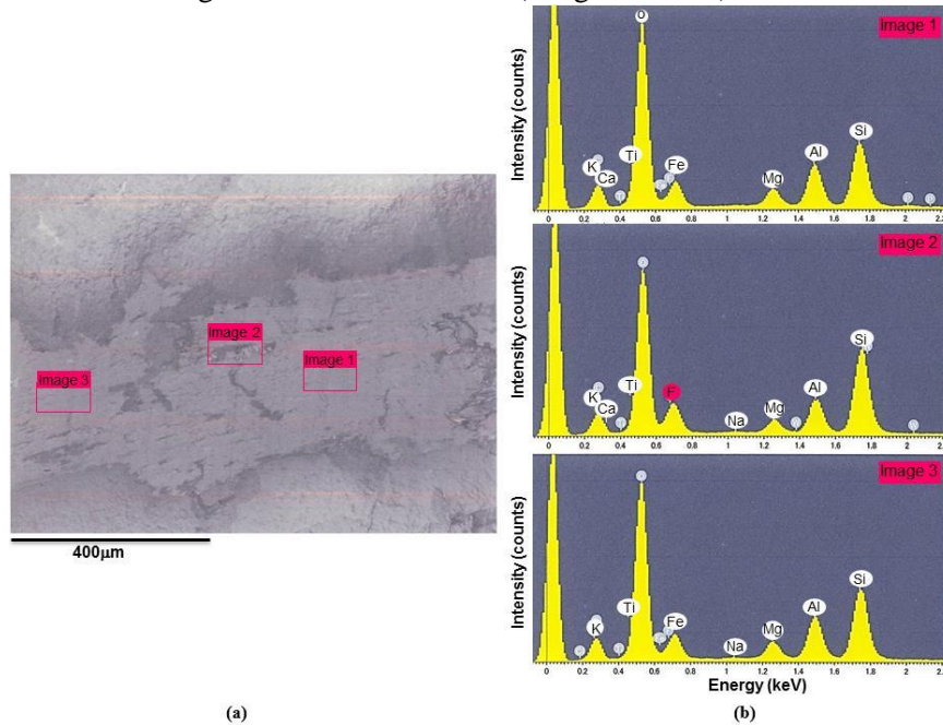
Figure 7. SEM-EDS results of an altered untreated granitic sample a) Scanning electron microscopy SEM image. b) Energy dispersive spectroscopy EDS of three different spectra
