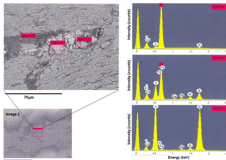
Figure 8. a) SEM image 2 of sample MIZ1-G3 b) Energy dispersive spectroscopy EDS of three different spectra, 70 \mu\text{m}
