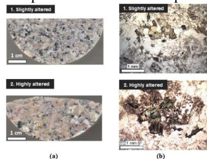
Figure 3. a) Scanning photo of rock specimens from MIZ-1 borehole. b) Optical microscopic photos of two rock specimens (Abdelgawad et al. 2009)
