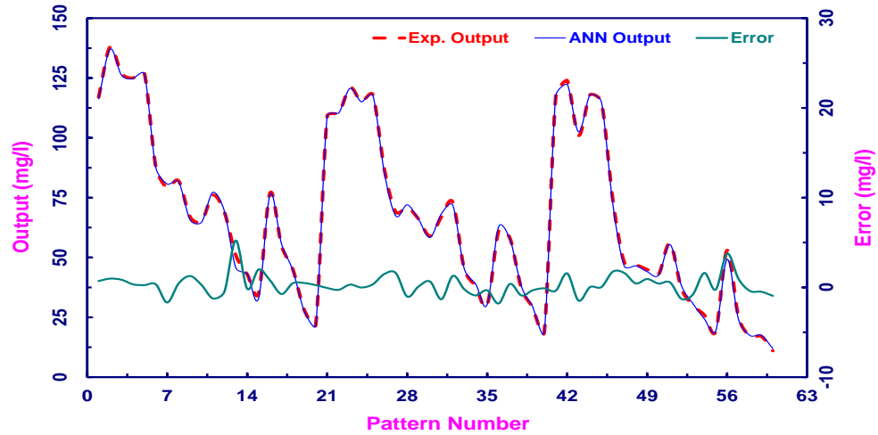
Fig. 10: Validation performance and error values of 60 patterns for TSS outputs
