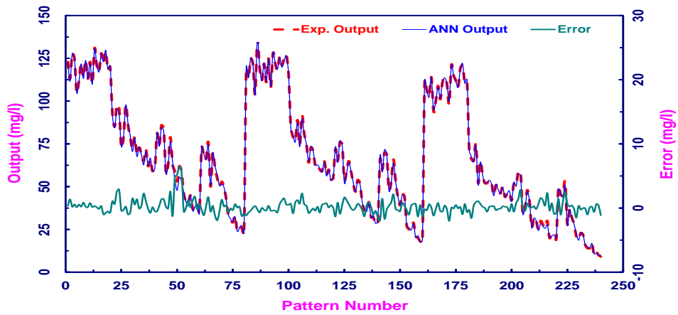
Figure. 6: Training performance and error values of 240 patterns for COD outputs
