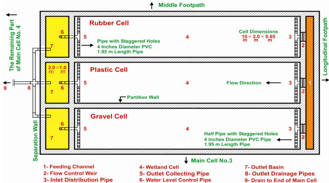
Figure. 1: Experimental setup for wetland cells
