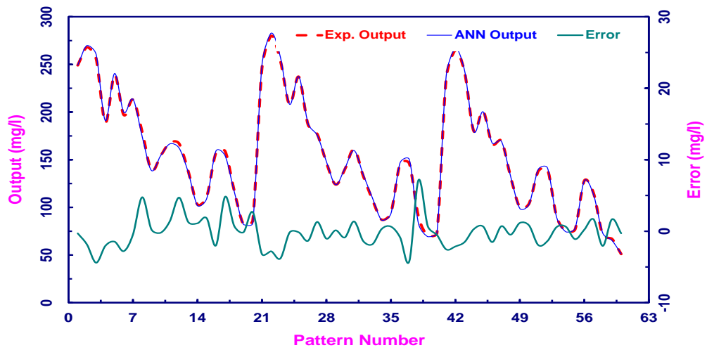
Fig. 9: Validation performance and error values of 60 patterns for COD outputs
