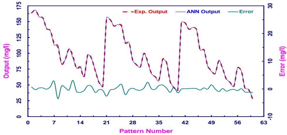
Fig. 8: Validation performance and error values of 60 patterns for BOD outputs
