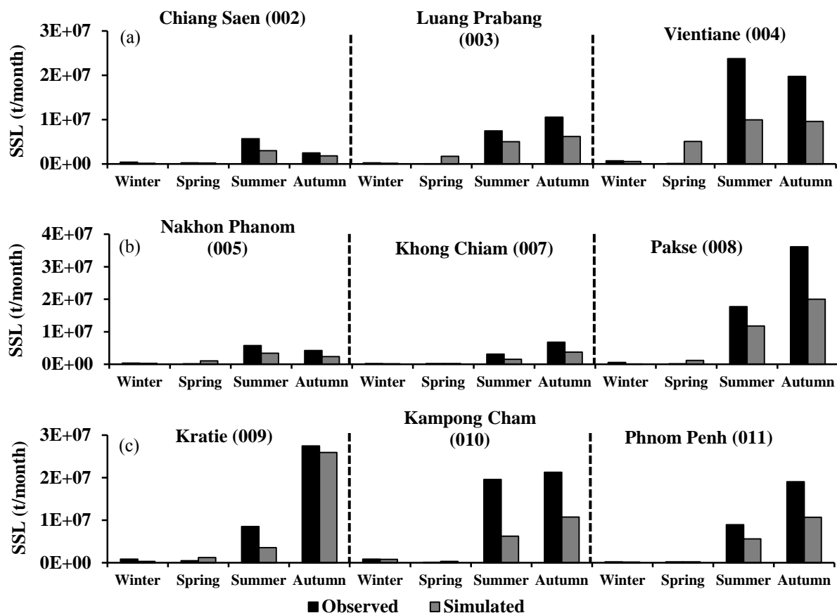
Figures 4. Seasonal change in the average SSL (a) upper region stations; (b) middle region stations; (c) lower region stations.
