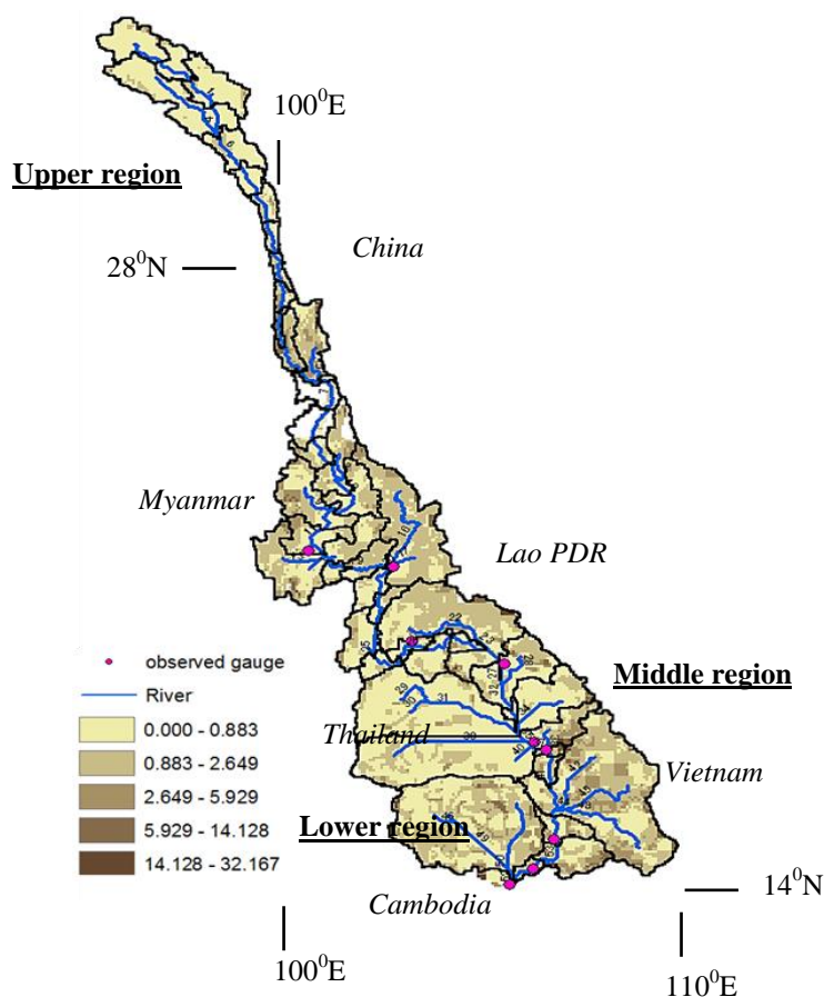
Figure 3. Average soil loss (ton ha -1 yr -1 )
