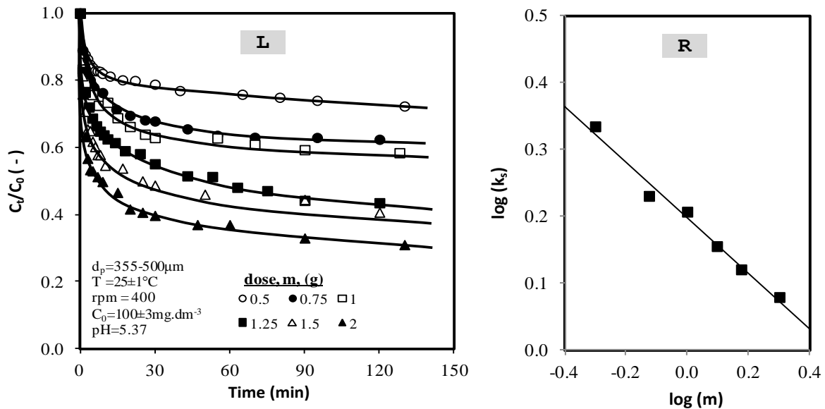
Fig. 4 (L) Typical time-concentration ratio at different adsorbent masses, (R) plot of \log k_s versus \log m for adsorption of methomyl onto CSAC.
