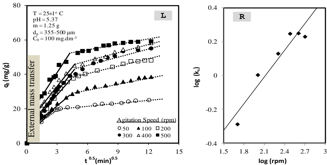
Fig. 5 (L) Plot of q_t against t^{0.5} for various agitation speeds, (R) plot of \log k_i against \log rpm during the adsorption of methomyl onto CSAC.
