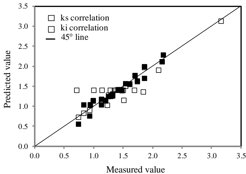
Fig. 7 Comparison between measured and predicted values for both correlations of surface and intraparticle diffusion models
