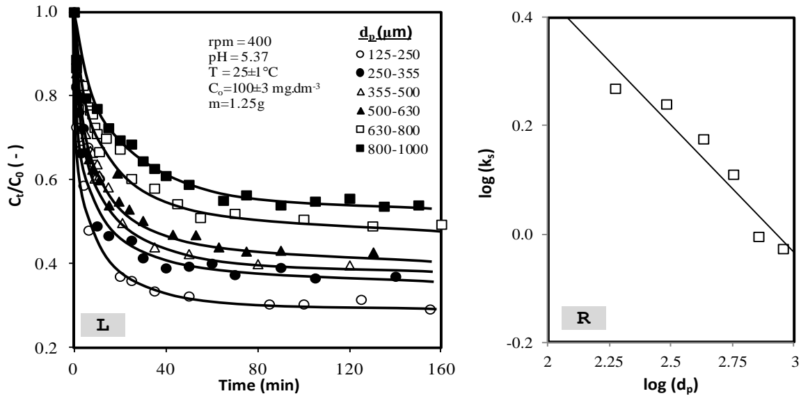
Fig. 3 (L) Typical time-concentration ratio at different particle size ranges, (R) plot of \log k_s versus \log d_p for adsorption of methomyl onto CSAC.
