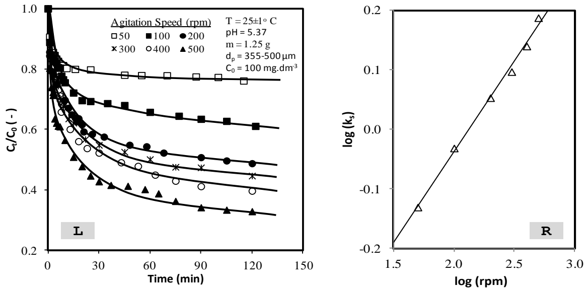
Fig.1 (L) Typical time-concentration ratio at different agitation speeds, (R) plot of \log k_s versus \log \text{rpm} for adsorption of methomyl onto CSAC.
