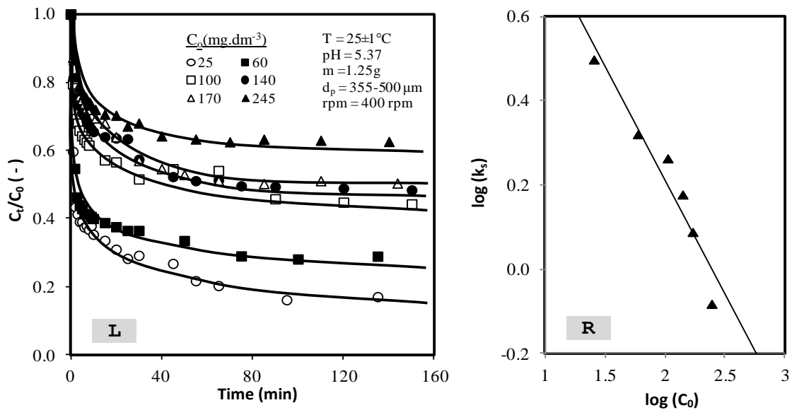
Fig.2 (L) Typical time-concentration ratio at different initial concentrations, (R) plot of \log k_s versus \log C_0 for adsorption of methomyl onto CSAC.
