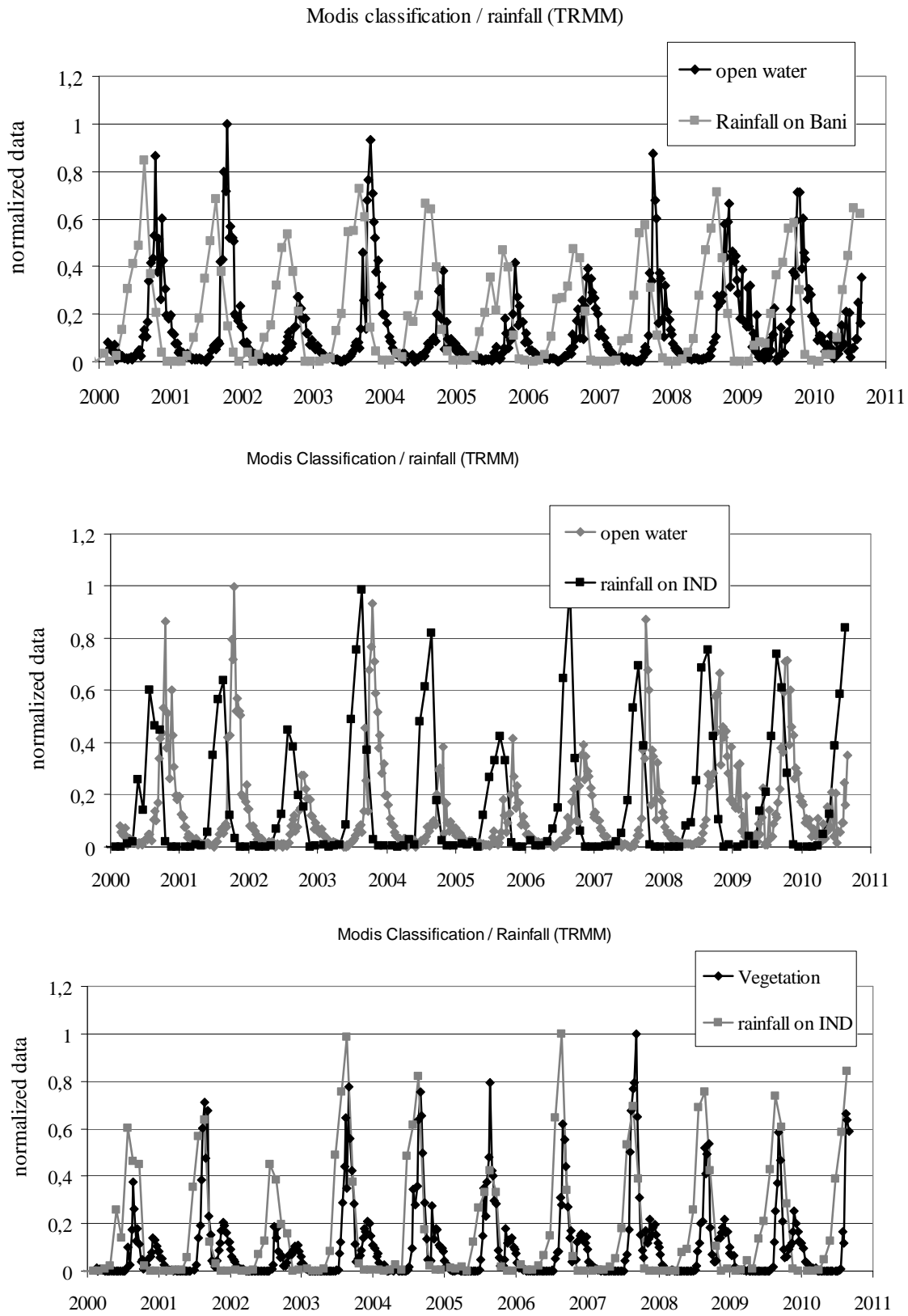
Fig. 2: Modis classification over the IND versus precipitation rate over the Bani River and the IND. (TRMM data set has been used for the computation of rainfall).
