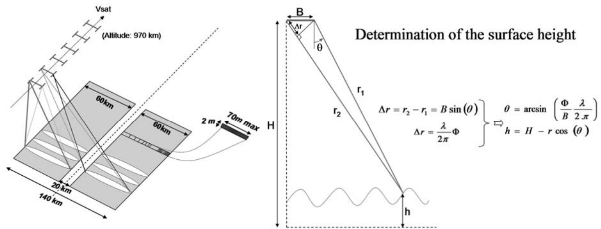
Fig. 7: SWOT mission. Radar Interferometry principle for the determination of water height over wide swath of 120 km along the orbital track of the satellite.
