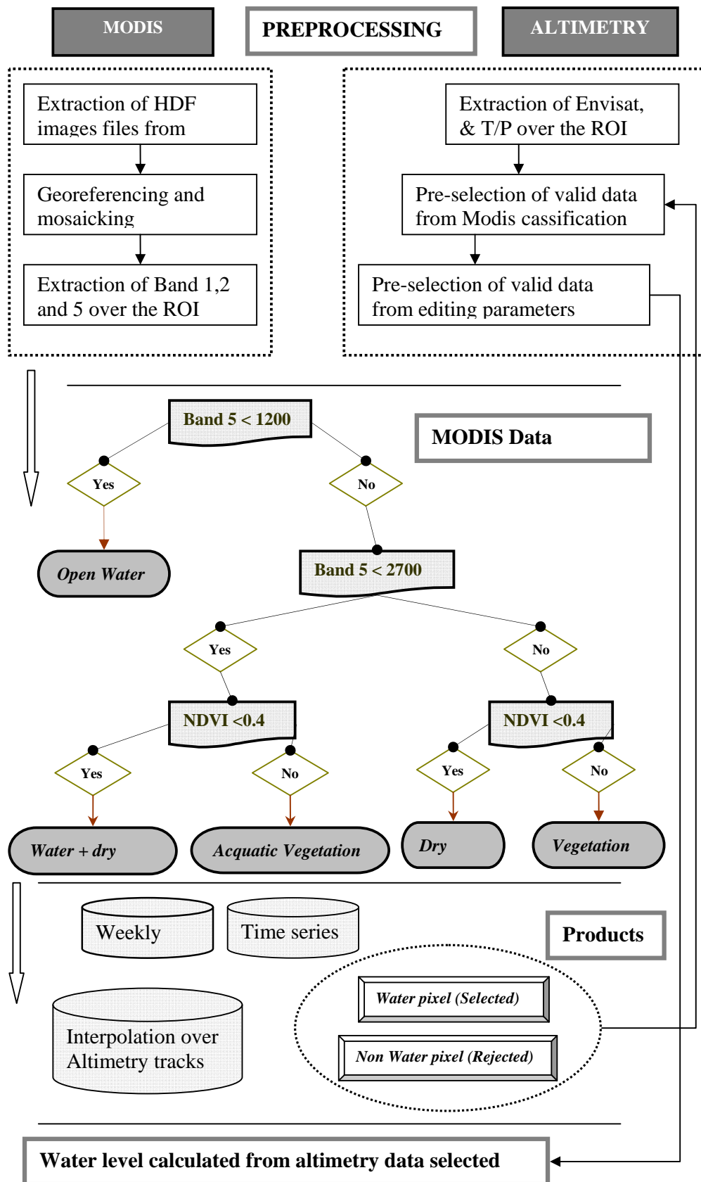
Fig. 1: Algorithm developed for the flood mapping from MODIS and water height determination from radar altimetry. Band Unit of reflectance is internal HDF-EOS data format specific to the Modis data and do not correspond to usual reflectance unit.
