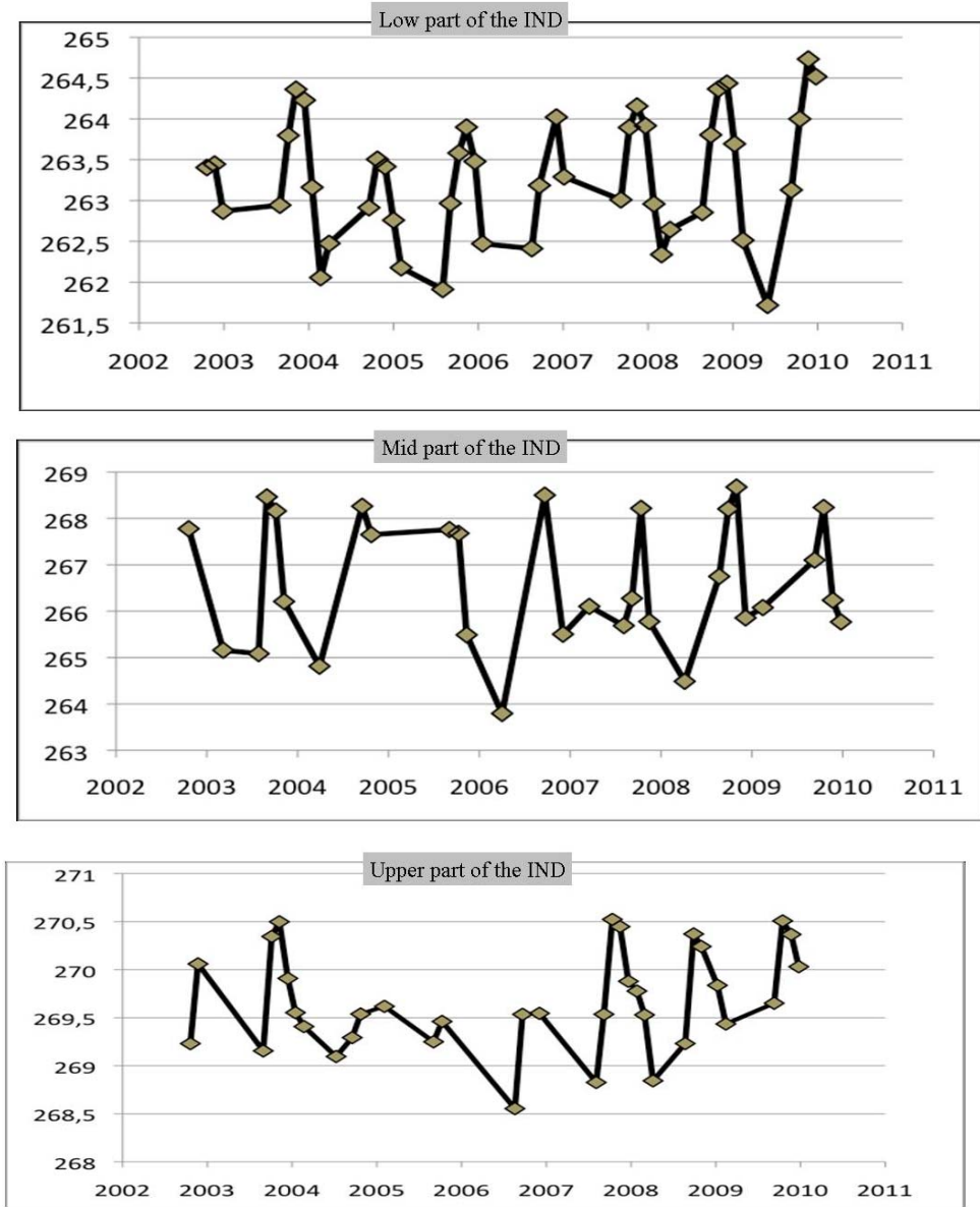
Fig. 4: level variations (m) over the IND from Envisat track n° 474
