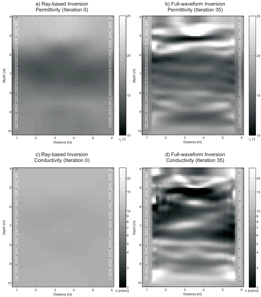
Figure 6. Distribution of (a) relative permittivity and (c) conductivity from ray-based inversions that are used as the initial model for the full-waveform inversion, (b) permittivity and (d) conductivity tomograms for iteration 35. Transmitter and receiver positions are indicated with crosses and circles, respectively. After Klotzsche et al., 2010 [25].
