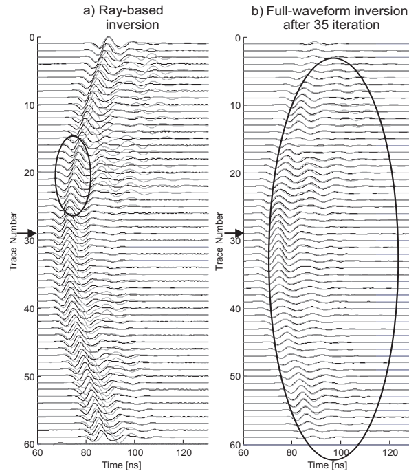
Figure 7. Comparison of observed (gray) and synthetic (black) traces: (a) Ray-based inversion results using initial source wavelet (normalized), (b) results after the full-waveform inversion (iteration 35). The ellipses indicate the areas of best fit between the traces. The arrows at trace number 29 indicate location of the transmitter. After Klotzsche et al., 2010 [25].
