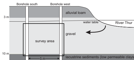
Figure 5. Simplified geological representation of the investigation site showing a three-layer structure: alluvial loam, gravel, lacustrine (clay) sediments (from top to bottom). Boreholes close to the river Thur; water table -4m depth. After Klotzsche et al., 2010 [25].
