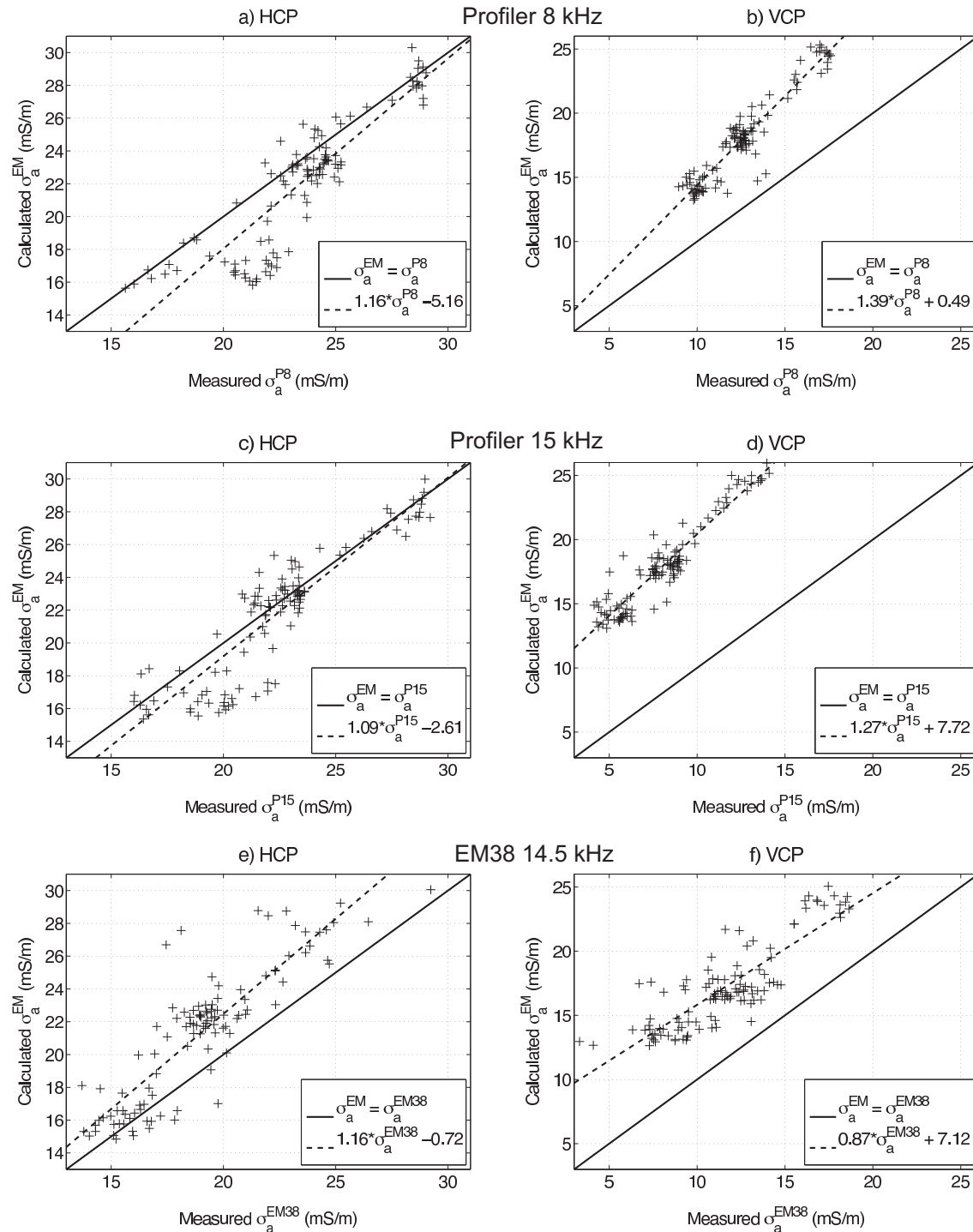
Figure 1. HCP and VCP scatter plots of measured \sigma_a versus synthetic \sigma_a for profiler 8 kHz (a,b) and 15 kHz (c, d) and EM38 (e, f), respectively. Dashed lines show the corresponding linear regressions. After Lavoué et al., 2010 [3].
