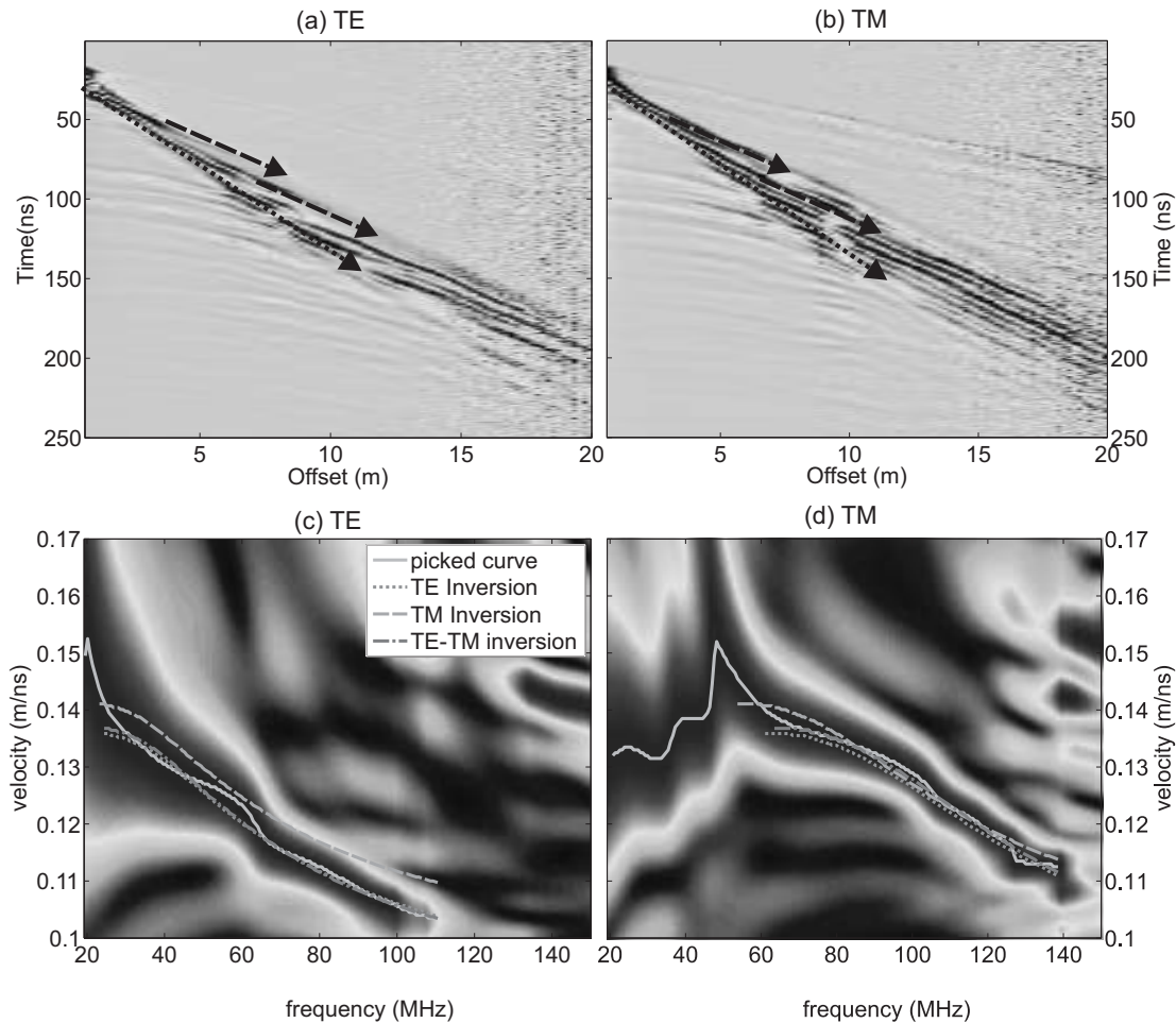
Figure 4. (a) TE and (b) TM CMP profiles measured after 72 mm rainfall over a dry sandy soil. The data are normalized to the maximum of each trace. The dotted arrow is the phase velocity, indicating the velocity with which the phases are traveling through the waveguide. Observed phase velocities are indicated by the dashed arrows. Corresponding (c) TE and (d) TM phase velocity spectra diagram of the broadside (TE) and endfire (TM) source-receiver setups, respectively.
