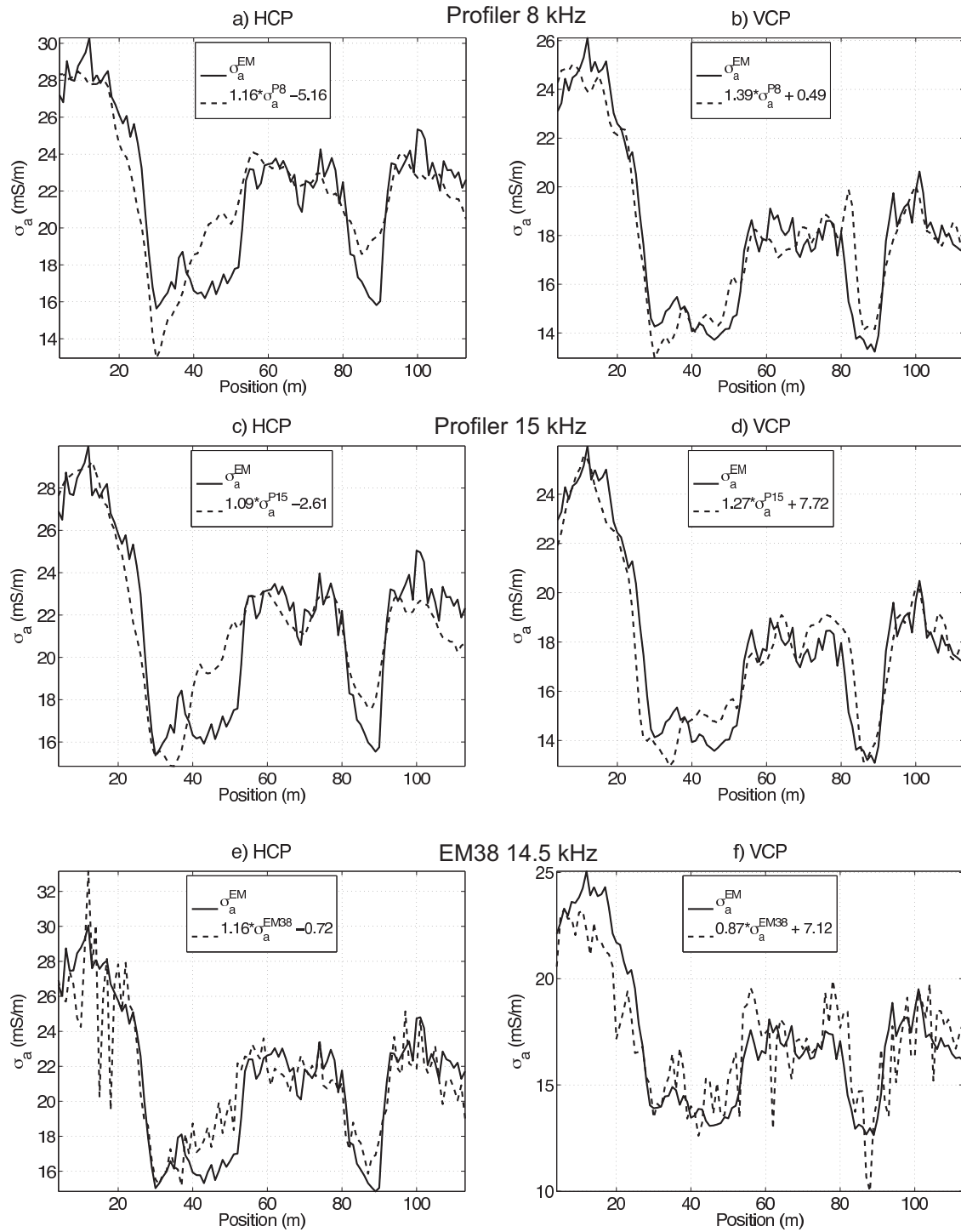
Figure 2. HCP and VCP EM-based calculated apparent conductivities (black) and calibrated values from measured apparent conductivities (dashed line) for profiler 8 (a, b) and 15 (c, d) kHz and EM38 (e, f), respectively. After Lavoué et al., 2010 [3].
