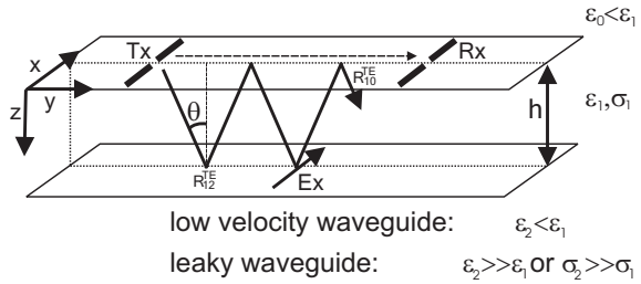
Figure 3. Diagram of the broadside (TE) source-receiver
