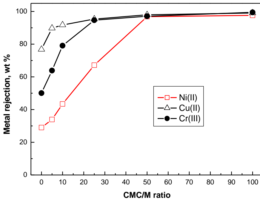
Figure 2. Effect of CMC concentration on the rejection of Ni(II), Cu(II) and Cr(III) from aqueous solutions using polyethersulfon ultrafiltration membrane. (pH = 7, p = 1 bar)
