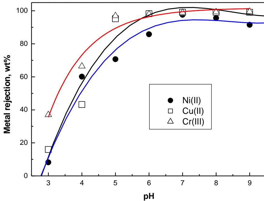
Figure 1. Effect of pH on the rejection of Ni(II), Cu(II) and Cr(III) from aqueous solutions using polyethersulfon ultrafiltration membrane. (CMC: M = 100, p = 1 bar)
