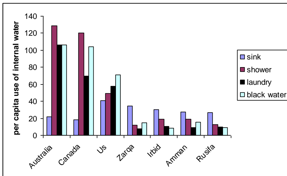
Figure 1. Comparison between the per capita rate of internal water consumption for the different internal water uses for Irbid, Rusaifa, Zarqa, Amman and other countries
