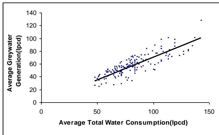
Figure 5. The average greywater generation versus average total household water consumption in (a) Irbid, (b) Rusaifa and (c) Zarqa
